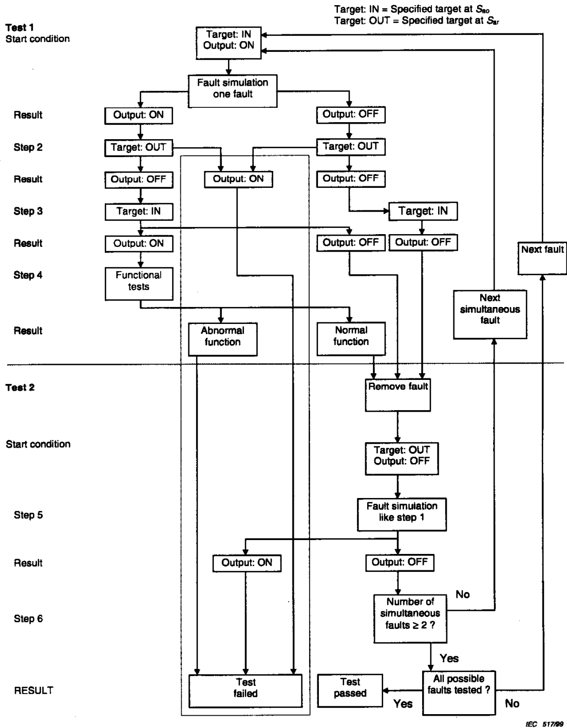
Figure A.3 – Test sequence for PDF-M
