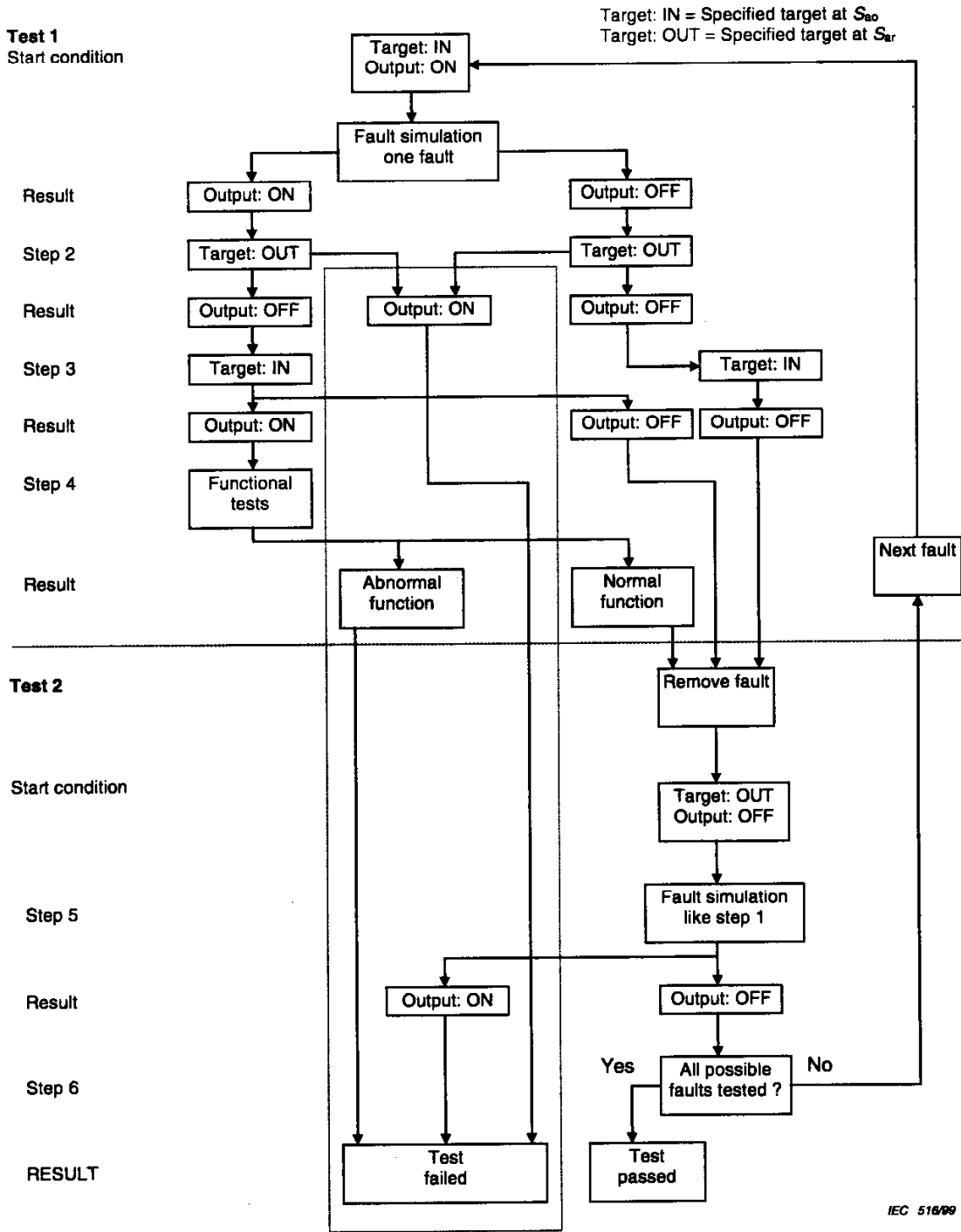
Figure A.2 – Test sequence for PDF-S
